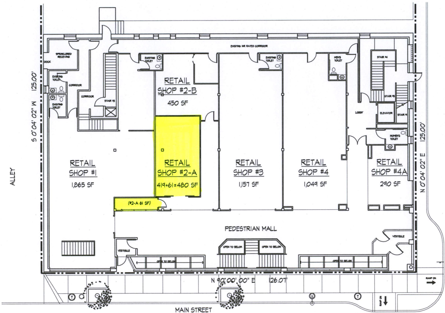
EXISTING FIRST FLOOR AND SITE PLAN DWG - P&P
